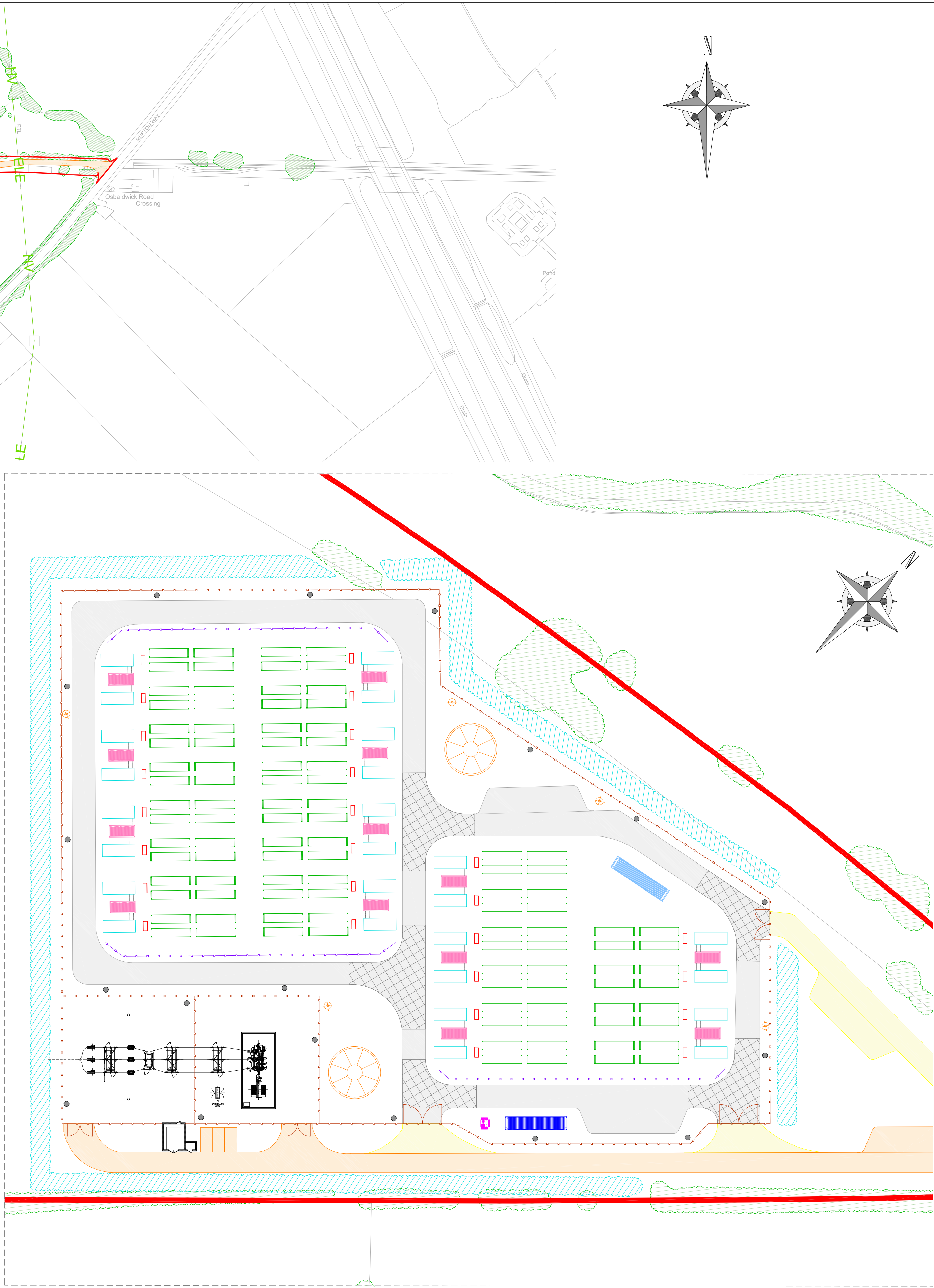
2 BATTERY SITE Scale: 1:500@A1
